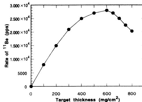
FIG. 3. Calculated rate of ^{11}\text{Be} (in particles per second) transmitted through LISE as a function of the Be target thickness for an incoming beam intensity of 2 \mu\text{Ae} and a momentum acceptance of 0.12%. The optimum thickness is found around 600 \text{ mg/cm}^2 .
